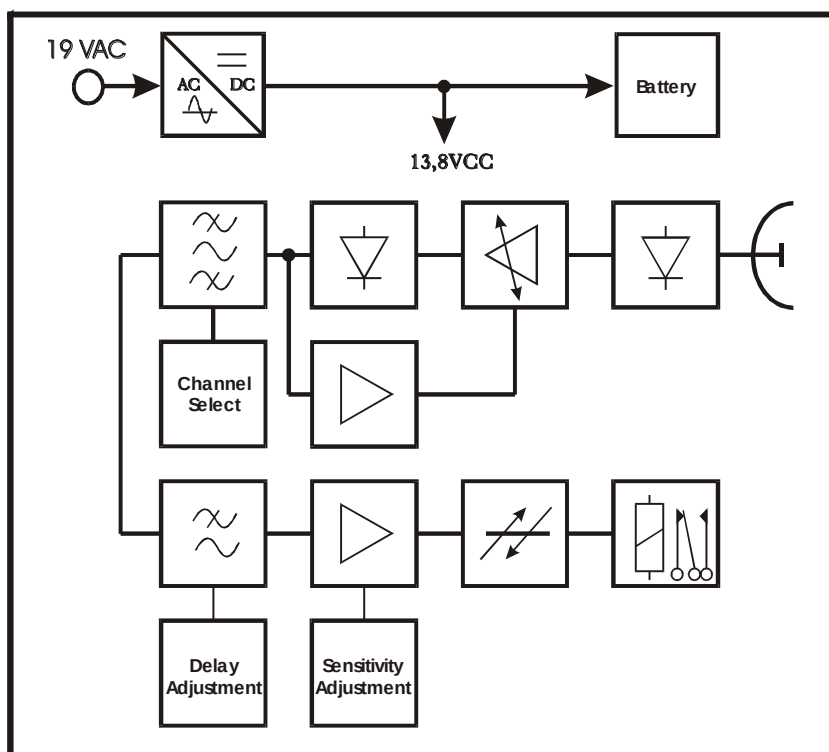
Ermo 482 Receiver Block Diagram
