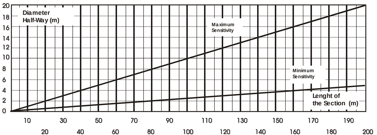
Figure 4 Diameter of sensitive beam at the half-section length (ERMO 482/ 80-120-200) (Free space)
