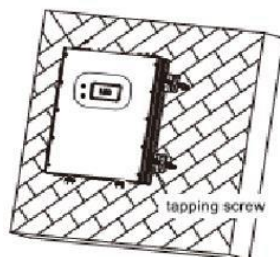
Hi20/Hi23 - 3S/5S/6S
